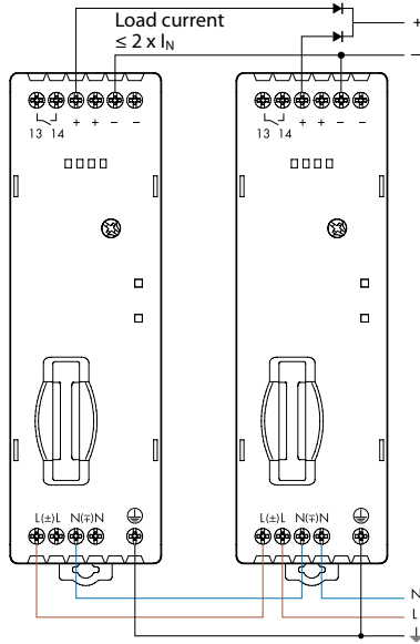
Parallel connection
