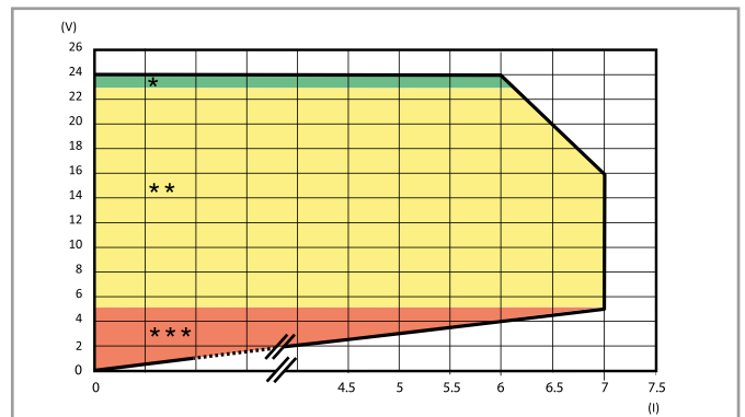
FB78-4 Output voltage vs output current (78.1D)
