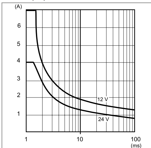
P78-2 Output peak current v time (78.36)
