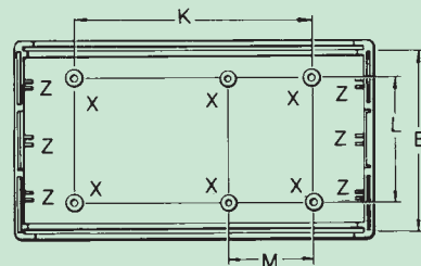
PLAN VIEW OF BASE AND TOP
