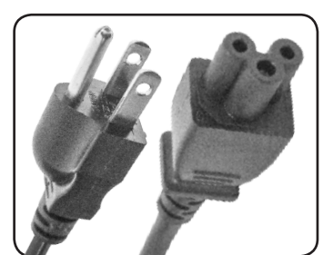
55-779-LENGTH 3-Prong AC Plug to Notebook (IEC C5) Power Cable. (18 gauge) AVAILABLE LENGTHS (FT.): 6 & 10.
