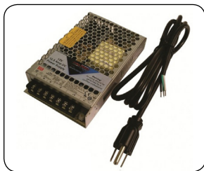
• 45-609-HG-UL (350W/29 Amp) • 45-610-HG-UL (150W/12.5 Amp) Single Output Slimline 12Vdc Switching Power Supply
