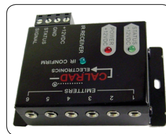
92-167 Send IR signals to 6 sources using a single emitter or 12 more sources if double IR emitters are used.
