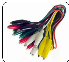
90-767 Test Clip Set, 10 leads, 15 in. long. Miniature insulated alligator clips & wire. 2 pcs of 5 colors: WH, BK, RD, GN, YL.
