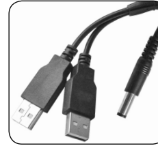
• 72-138-2.1 (2.1mm) • 72-138-2.5 (2.5mm) Dual USB (Type A) to Coaxial Plug. Enables power to a 5Vdc device. Up to 1 Amp.
