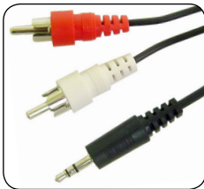
55-899-LENGTH 3.5 mm Stereo male plug to two RCA Male plugs. AVAILABLE LENGTHS (Ft.): 3, 6, 12 & 25.
