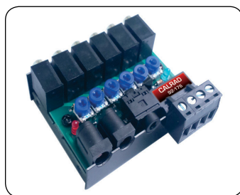
92-176 6 Port Amplified IR Distribution Block with Individual Signal Controls
