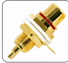
30-300-COLOR RCA chassis mount Audio Jack. Fits 5/16" hole. AVAILABLE COLOR BAND ID: BK, BU, GN, OR, RD, WH & YL
