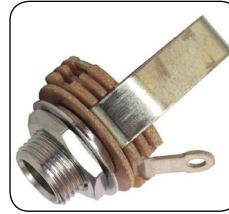
• 30-400 (Stereo) • 30-411 (Mono) 3 Circuit 1/4" Open, Audio Jack. 0.36" hole size.
