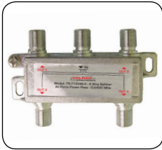
75-713-HG-OUTPUT Digital Splitter, All Ports Power Pass, 5-2400 MHz AVAILABLE OUTPUTS: 2, 3, 4, 6 & 8.
