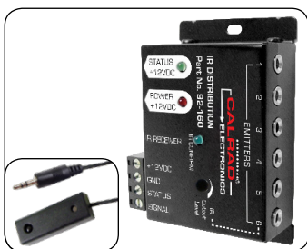
92-160 (6 Ports) IR Kit Distribution System with IR emitter gain control on port 6 only. INCLUDES: 3 x IR Emitters, 1 x Distribution Block, 1 x Surface Mount Receiver, 1 x 12Vdc, 300ma Power Supply
