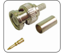
75-611 (50 ohm) 75-607 (75 ohm) BNC crimp for RG-58 cable. 3 piece.
