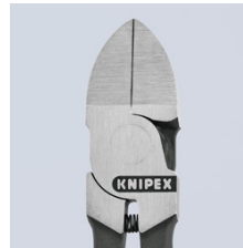
Extended cutting edge (5 mm) - improved transmission (+ 25 %)
