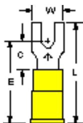
MVU10-6FB 6 12-10
