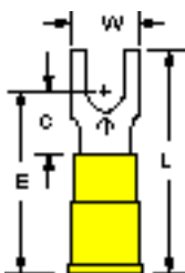
MVU10-8FB 8 12-10
