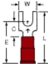
MNG18-8FB Stud Size 8 Wire Range 22-18
