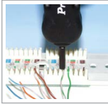
Punch and cut cable terminals
