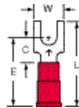
MV18-8FB Stud Size: 8 Wire Range: 22-18
