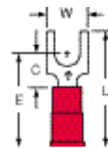
MV18-10FB Stud Size: 10 Wire Range: 22-18
