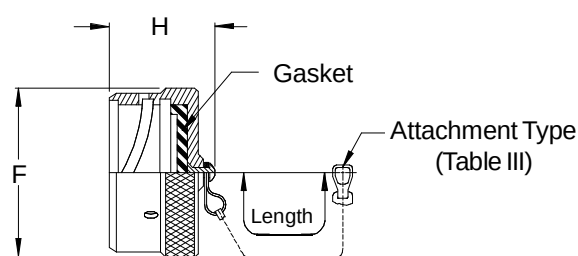
660-018 Receptacle Cover
