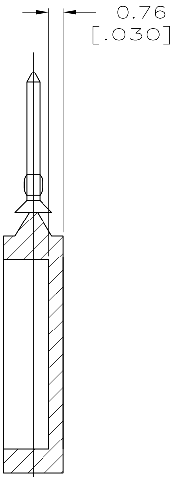
SECTION B-B OPTIONAL CONSTRUCTION 2 PLC
