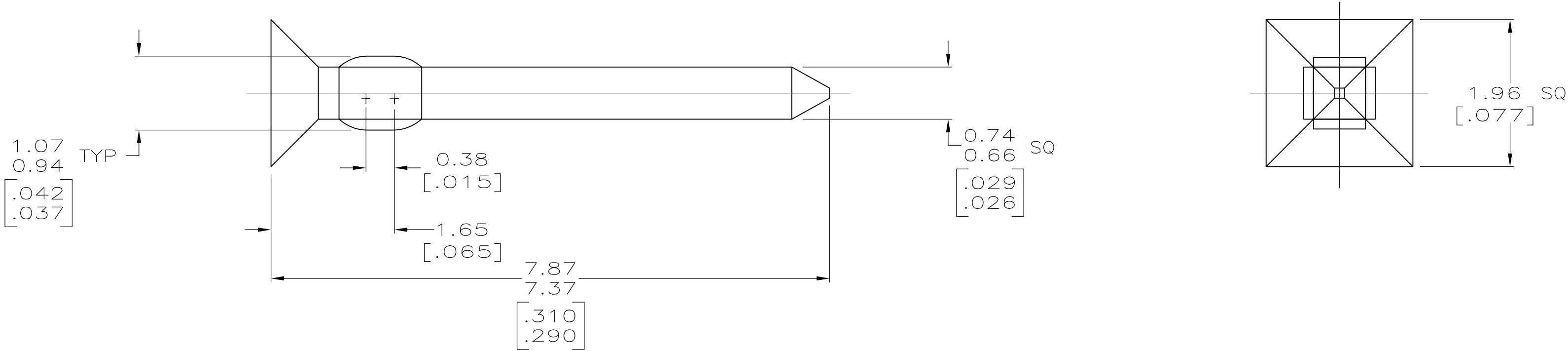
DETAIL A SCALE 20:1 ROTATED 90° CW
