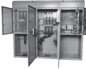
600V, NEMA Size 8, Synchronous Starter
