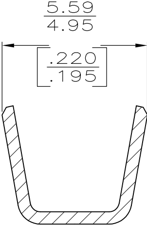
SECTION A-A SCALE 8:1
