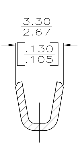
SECTION B-B SCALE 8:1
