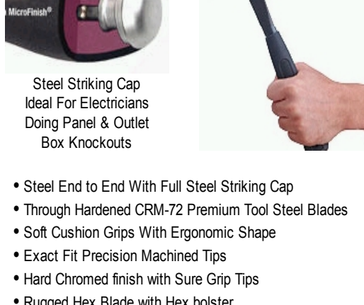
Cushion Grips, Hex Blade, Hex Bolster, Steel Cap
