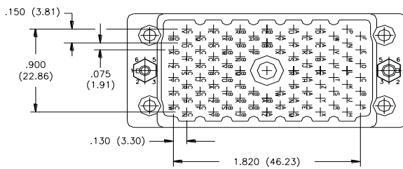
90 PIN PLUG
