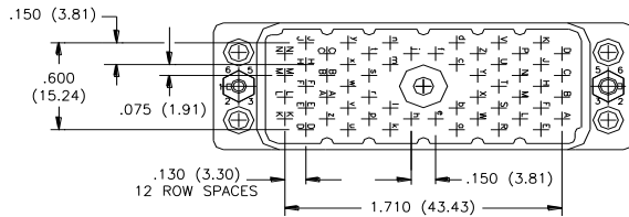
56 PIN PLUG
