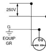
6-15R
