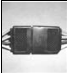
2512F 4-Pole moisture proof style trailer connector for C.B. radio hook-up, utility lights & accessories. Polarized plugs & color-coded.
