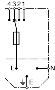
with internal connections Voltage selector 4-positions, 1-pole
