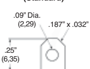
S Solder Eye & Quick Connect (Standard)
