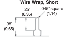
P 1 Printed Circuit and Wire Wrap, Short
