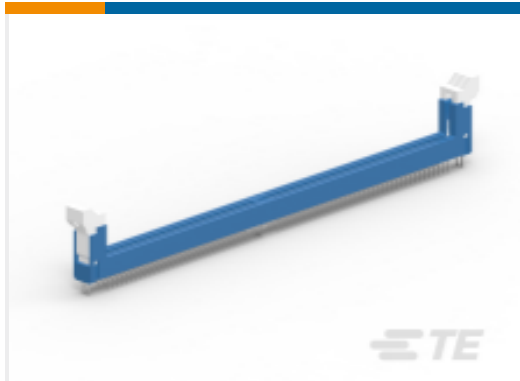
TE Model / Part #2308107-6 DDR4 DIMM 288 PIN TH TYPE
