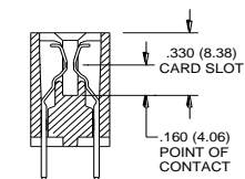
DUAL ROW
