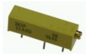
343 Series Trimmer, 500 kOhm, 0.75 W, 20 Turns, Rectangular Body, Horizontal Shaft
