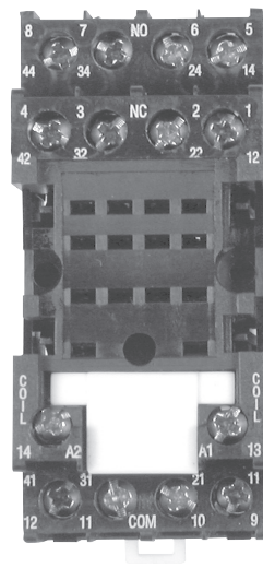
600-3-0018 DIN Rail or Base Mount, 4PDT, Miniature Relay Socket 30mm (W) x 71.5mm (T) x 29mm (D)
