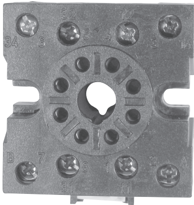
600-3-0013 DIN Rail or Base Mount, 8 Pin 43.5mm (W) x 43.5mm (T) x 20mm (D)
