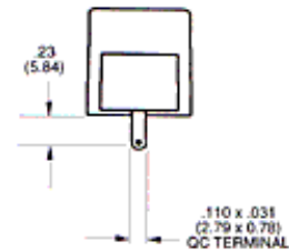
3 - Quick Connect .110"
