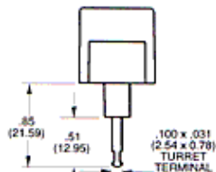
2 - Turret Type Solder Terminal
