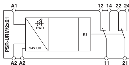
Block diagram
