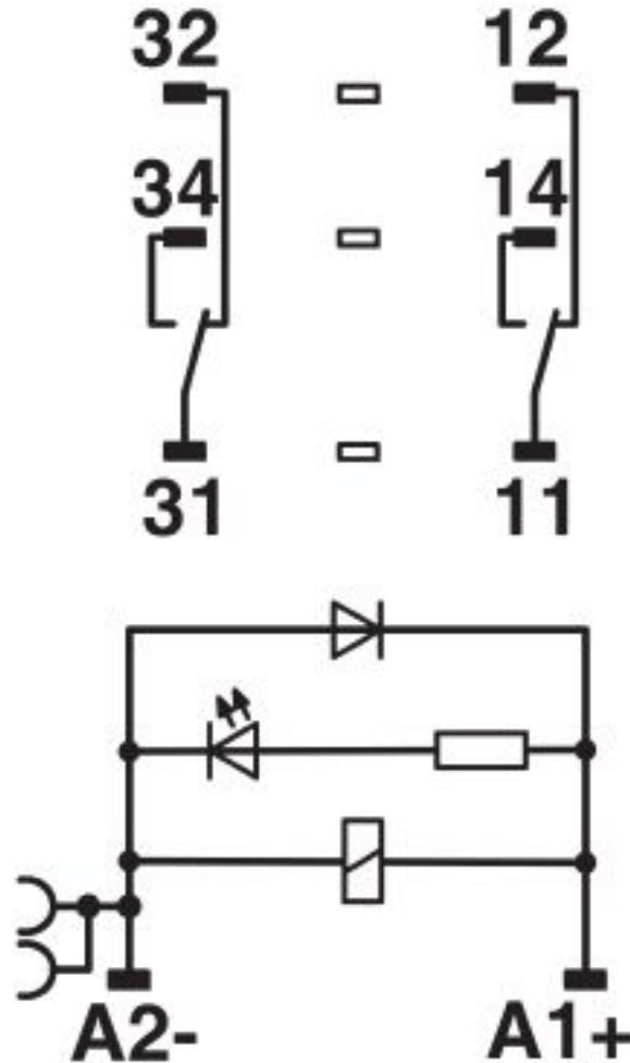
Circuit diagram
