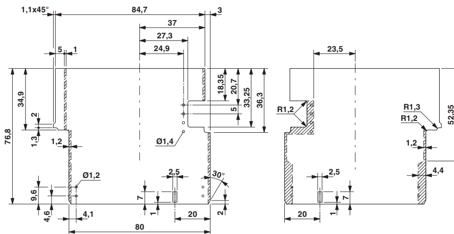
Dimensional drawing
