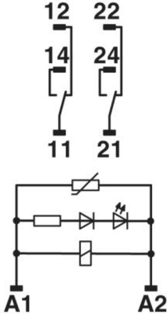
Circuit diagram
