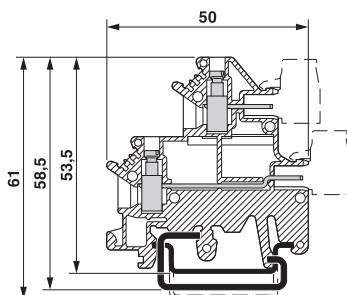
Dimensional drawing
