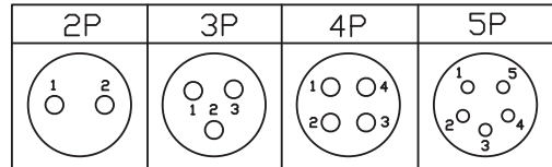
Pin Layout
