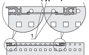
Cover plate for insertion in horizontal rails (type L)
