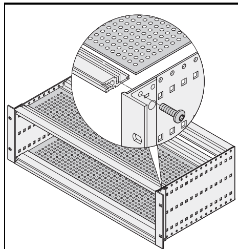
Cover plate for insertion in horizontal rails (type L)
