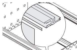
Stainless steel EMC gasket between front panel/rear panel and horizontal rail
