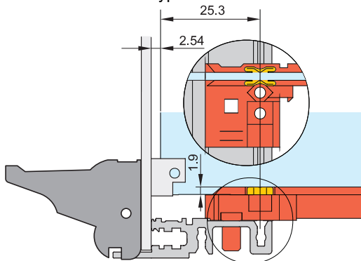
Guide rails on horizontal rail type H
