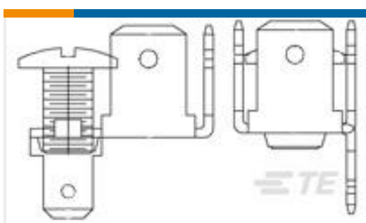
TE Part #8-2232265-3 POWER TRIPLE LOCK GLOW WIRE PLUG
