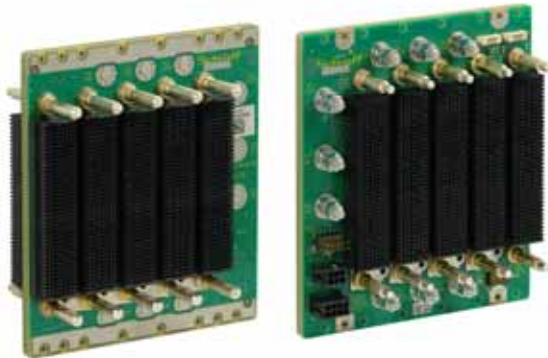
VPX backplane, 3 U, 5 slot, with rear I/O
