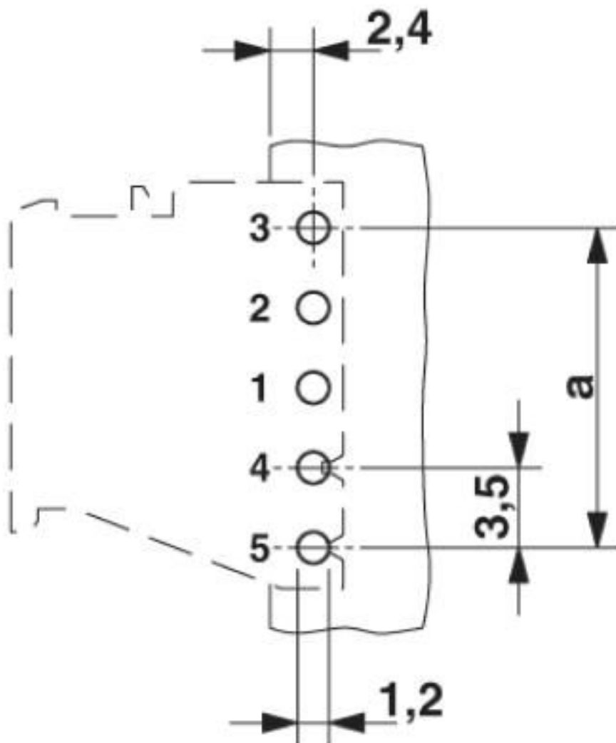
Drilling diagram
