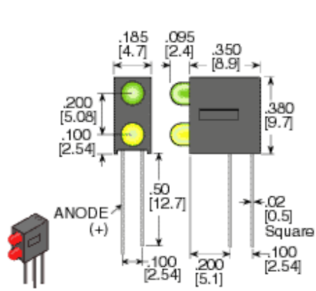
(21PCT120T4-G/Y Pictured) Dimensions in inches [mm]
