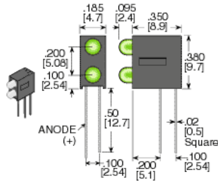
(21PCT120T3-0002 Pictured) Dimensions in inches [mm]
