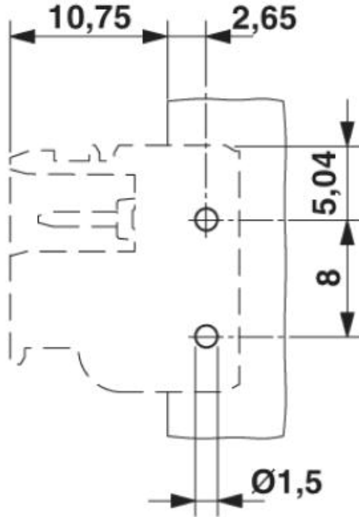
Drilling diagram
