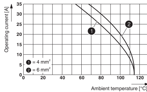
Derating diagram: HC-HS...S series
