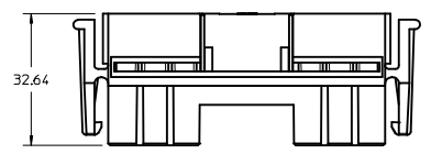
MAIN HOUSING
