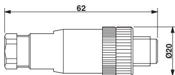
Plug, M12 x 1, straight, shielded
