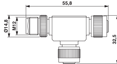
Dimensional drawing
