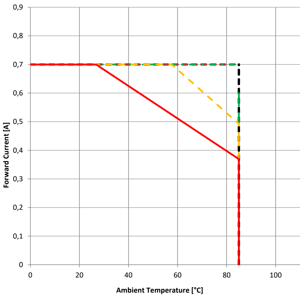
Derating Curve:
