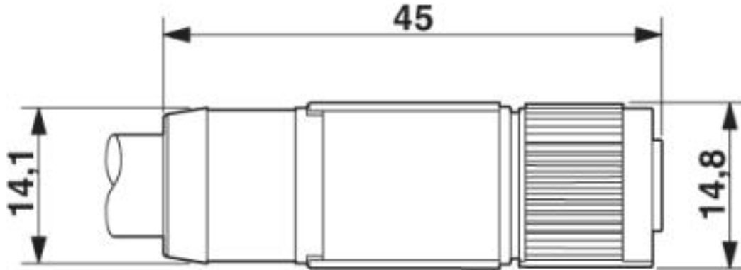
Dimensional drawing
