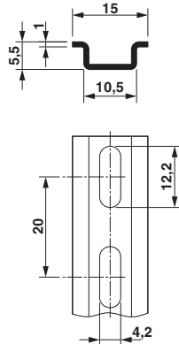
Dimensional drawing
