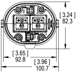
Front View - H02
