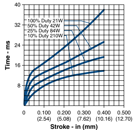
Size 5EC— Typical Speed @ No Load, 20°C
