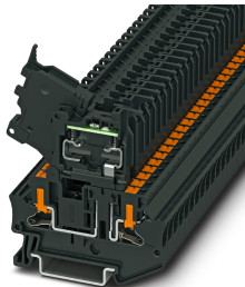
Lever-type fuse terminal block, black, for 5 x 20 mm G fuse inserts, with LED for 24 V DC
