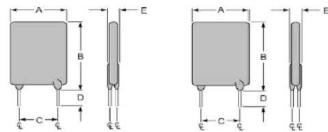
Fig.3 Lead Size: 20AWG Ø0.81 mm Diameter
