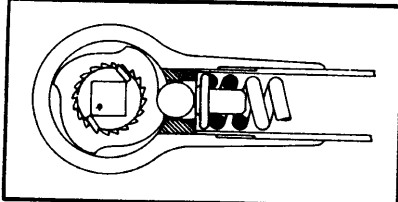
Working principle of Torqueleader Torque Safe
